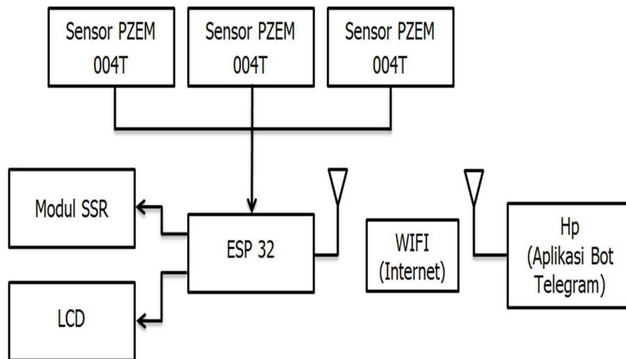
Gambar 1. Blok Diagram Sistem Monitoring Tegangan 3 phase
