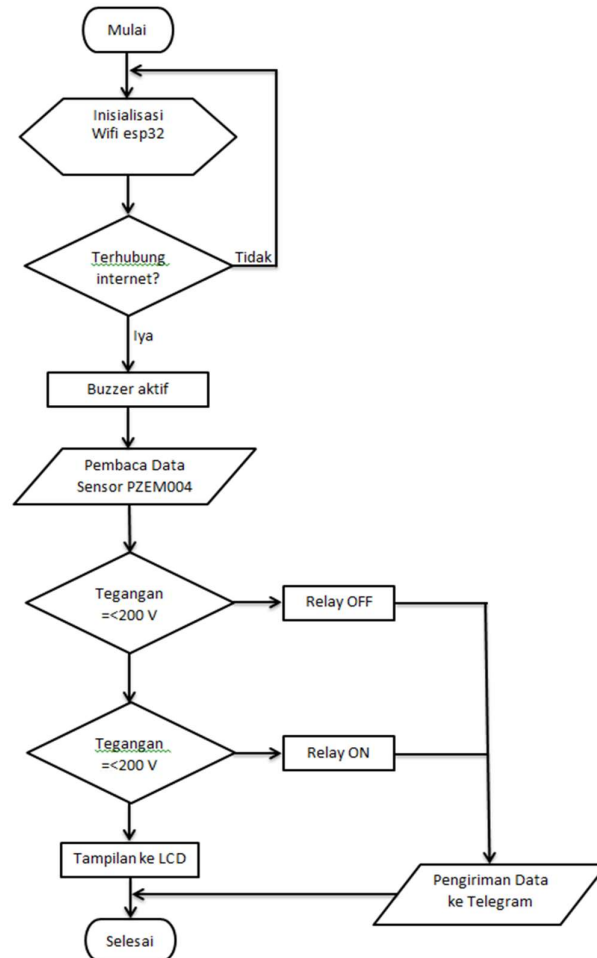
Gambar 3. Flowchat Sistem Monitoring Tegangan Tiga Phase dan Kendali On/Off Pompa
