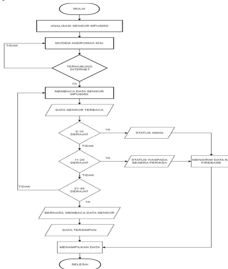
Gamba 6. Flowchart
