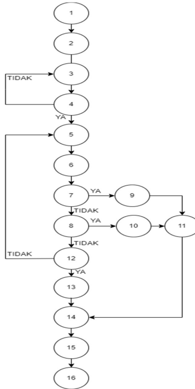
Gambar 7. Flowgraph
