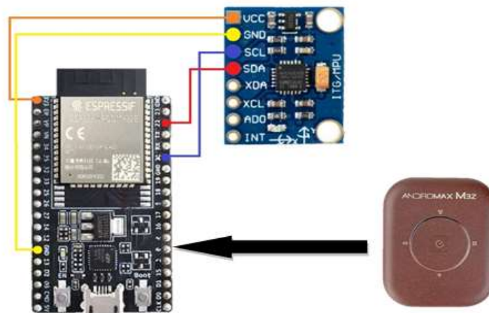
Gambar 1. Rancangan Hardware
