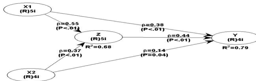
Gambar 2. Model Hipotesis
